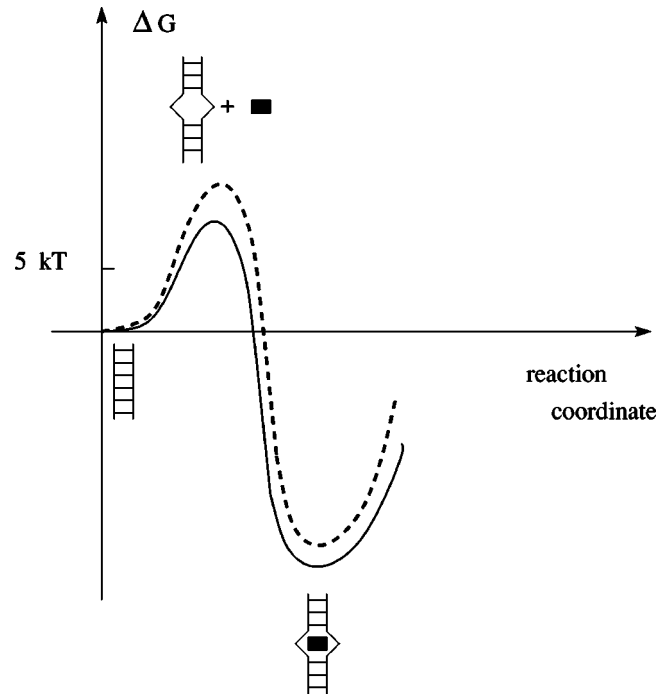
FIG. 3. Schematic drawing showing the modification of intercalation energy barrier and energy well coming from mechanical contribution \Delta\Delta G . The units are realistic: the barrier is of order 7kT ; the excess energy is there about 2-3kT . The binding energy is of order -20kT ; the excess energy is there about 1-2kT (the intercalated site is smaller than the “open” site required in the first step of intercalation, which reduces \Delta\Delta G into \Delta\Delta G_{int} ) [18,19].
