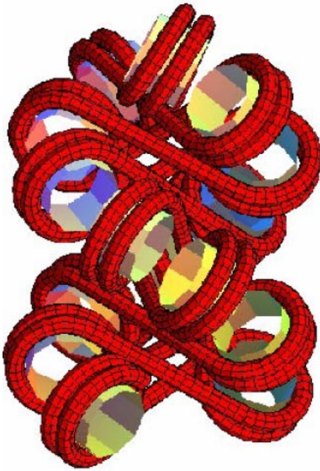
FIG. 2. (Color online) Proposed model of condensed chromatin, locked by interactions between stacked nucleosomes and presumably also by histone tails [9]. The chromatin fiber axis is here vertical.
