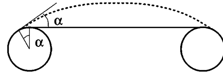
FIG. 4. Buckling of the linker is possible only when the linker ends are allowed to unwrap from the nucleosomes. Unwrapping by 5 bp on each side is enough to accommodate a buckling angle \alpha = 20^\circ , associated with \Delta l/l = 0.03 ; within these bounds, the situation is mechanically equivalent to hinged ends ( \nu = 1 ).
